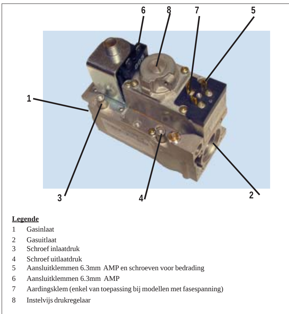
Figuur 10b : HONEYWELL gasklep (type 035-2 -> 100-2)
